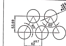
DETAIL OF TUBE PLATE HOLES
