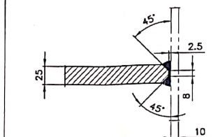
DETAIL AT "A" EDGE PREPARATION OF TUBE PLATE
